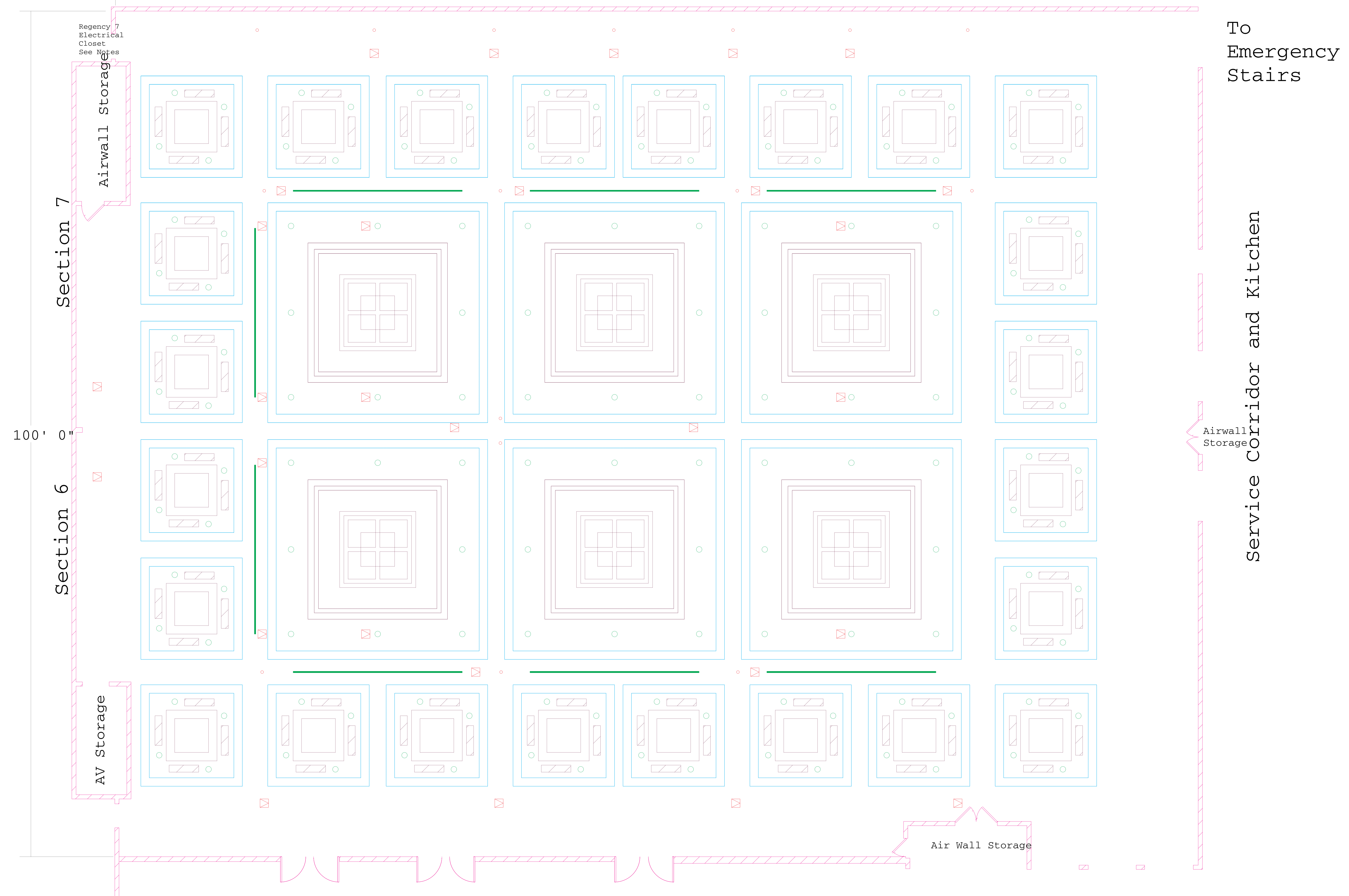
Plan View Regency Ballroom Sections 5, 6 and 7
